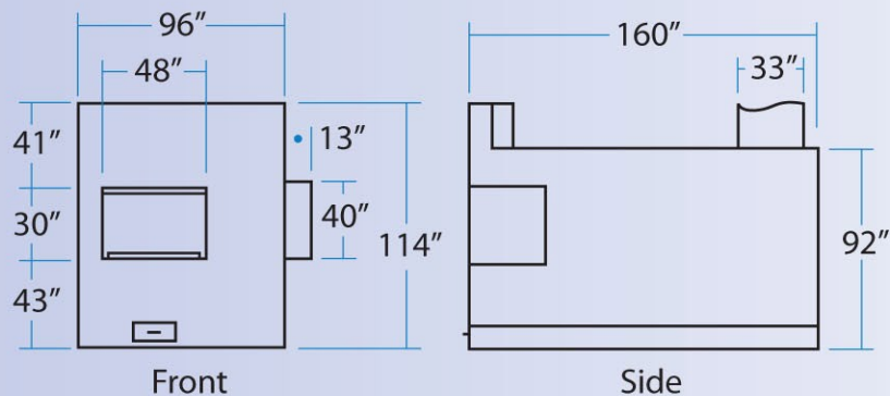
CU-200 Exterior Dimensions
