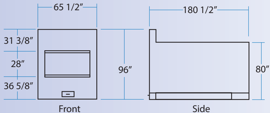
CU-150 Exterior Dimensions
